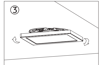
③ Press the light to fit the bracket and Rotate clockwise.
