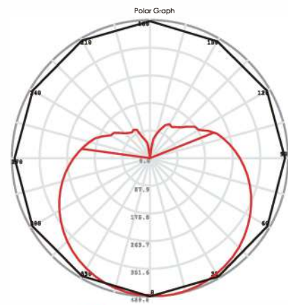
2D Light Intensity Distribution Curve
