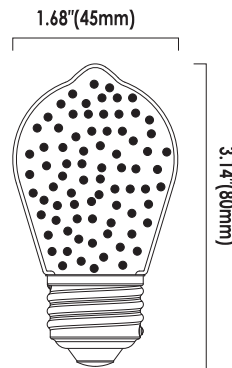
VO-FST14W5.5-26-30-D-M
