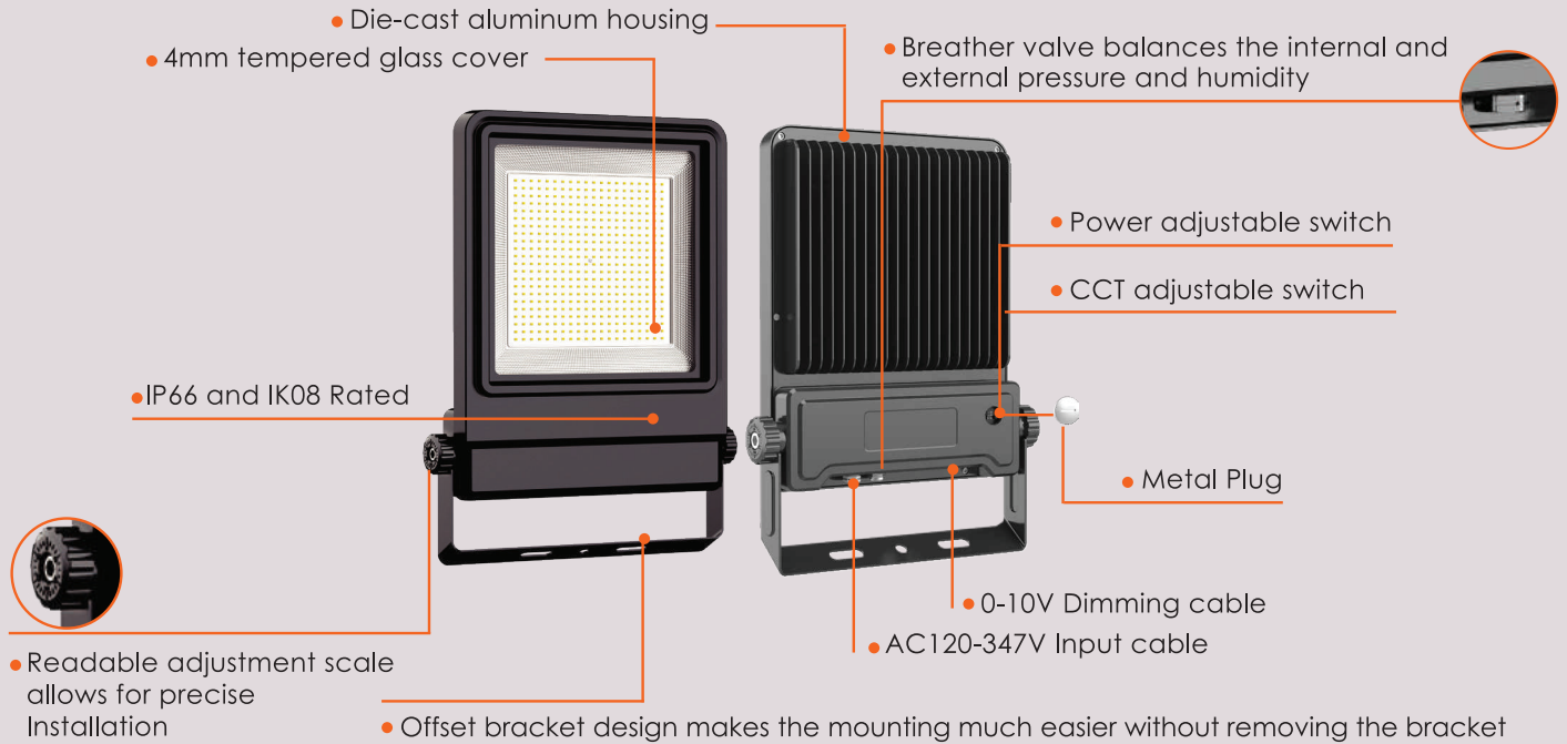
ISL-FL02-A-200/250/300W
