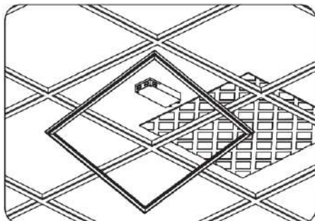
c) Remove the plasterboard and install the fram light in the T-bar.
