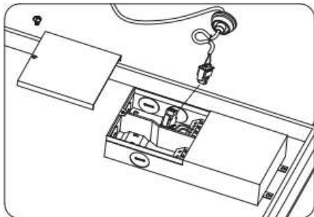
a) Screw off the cover of the driver knock off one of the knock-out on the driverz
