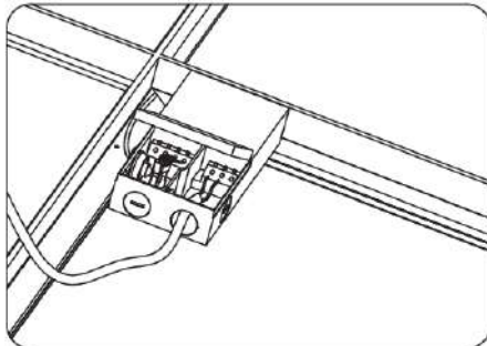
d) Take off knock-out one the other side, connect all wires with the AC input properly according to the labels on wires.
