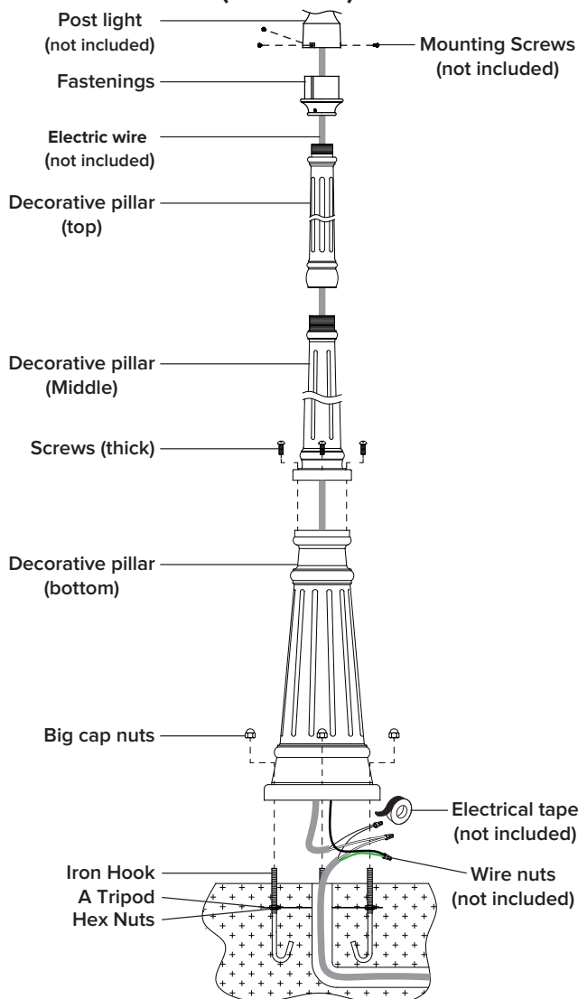
Decorative Pillar (TOP)
